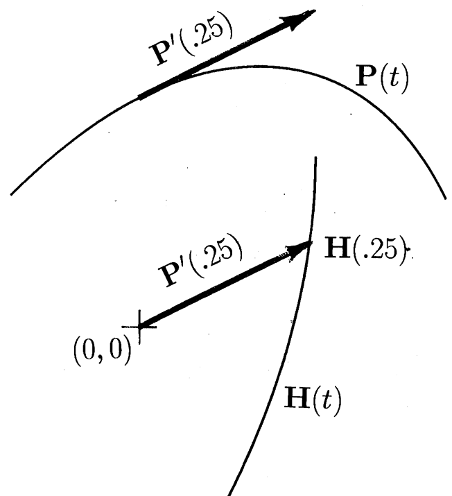
Figure 17. Tangent vector
