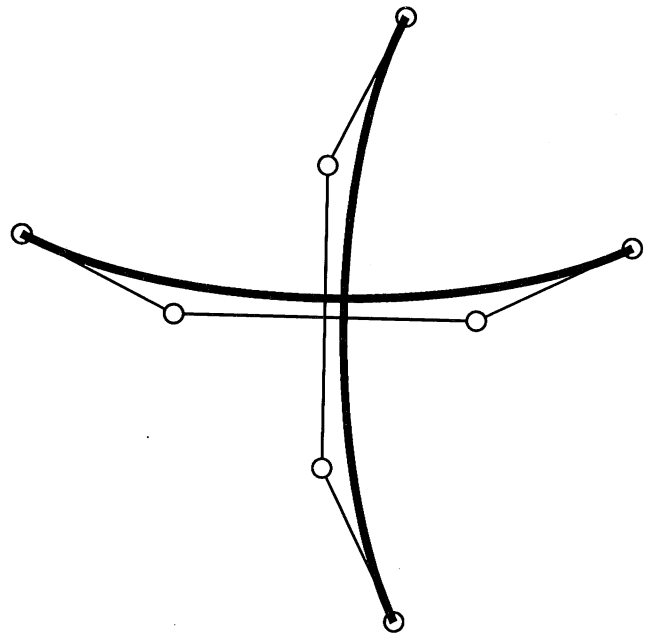
Figure 29. Degree-three example
