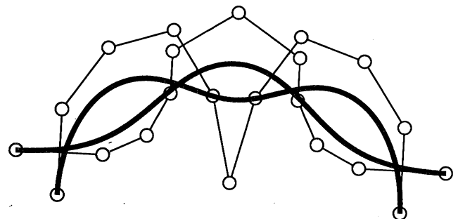
Figure 31. Degree-ten example
