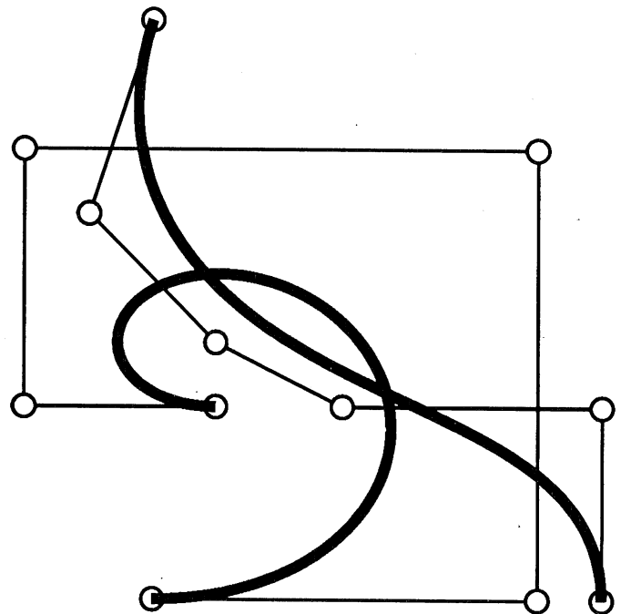
Figure 30. Degree-five example
