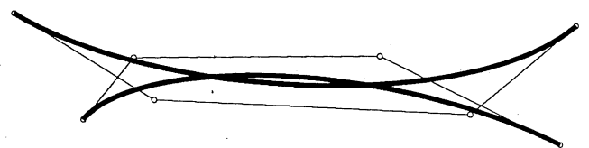
Figure 9. Two intersections
