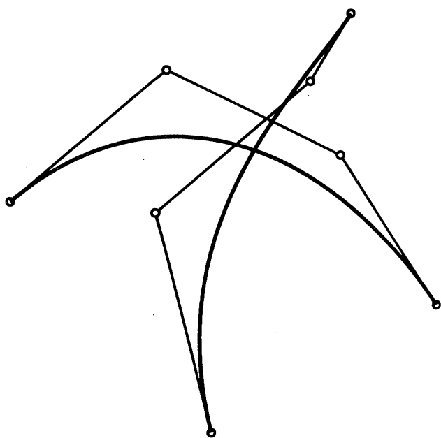
Figure 28. Degree-three example
